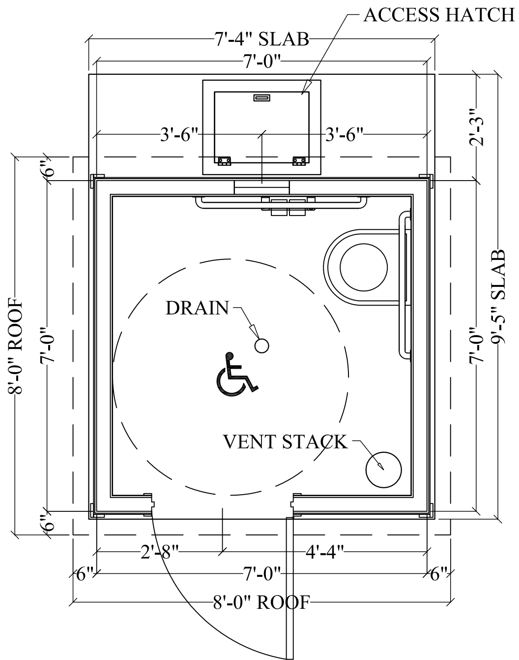
FLOOR PLAN
