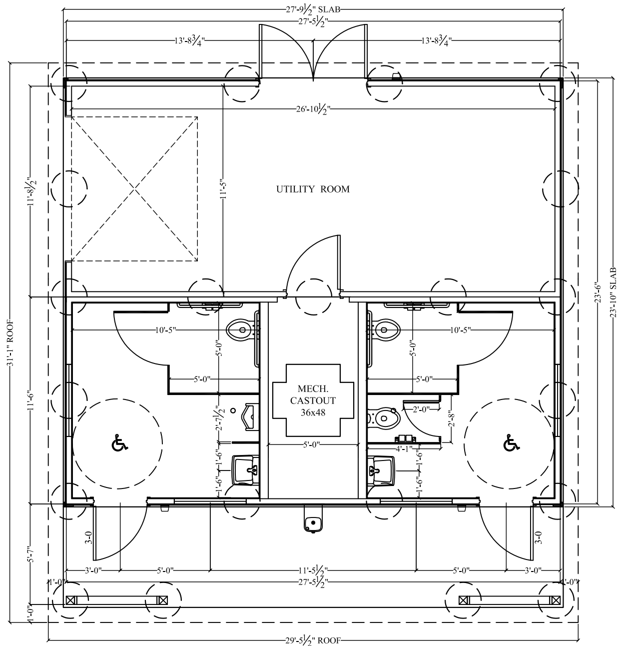
FLOOR PLAN
