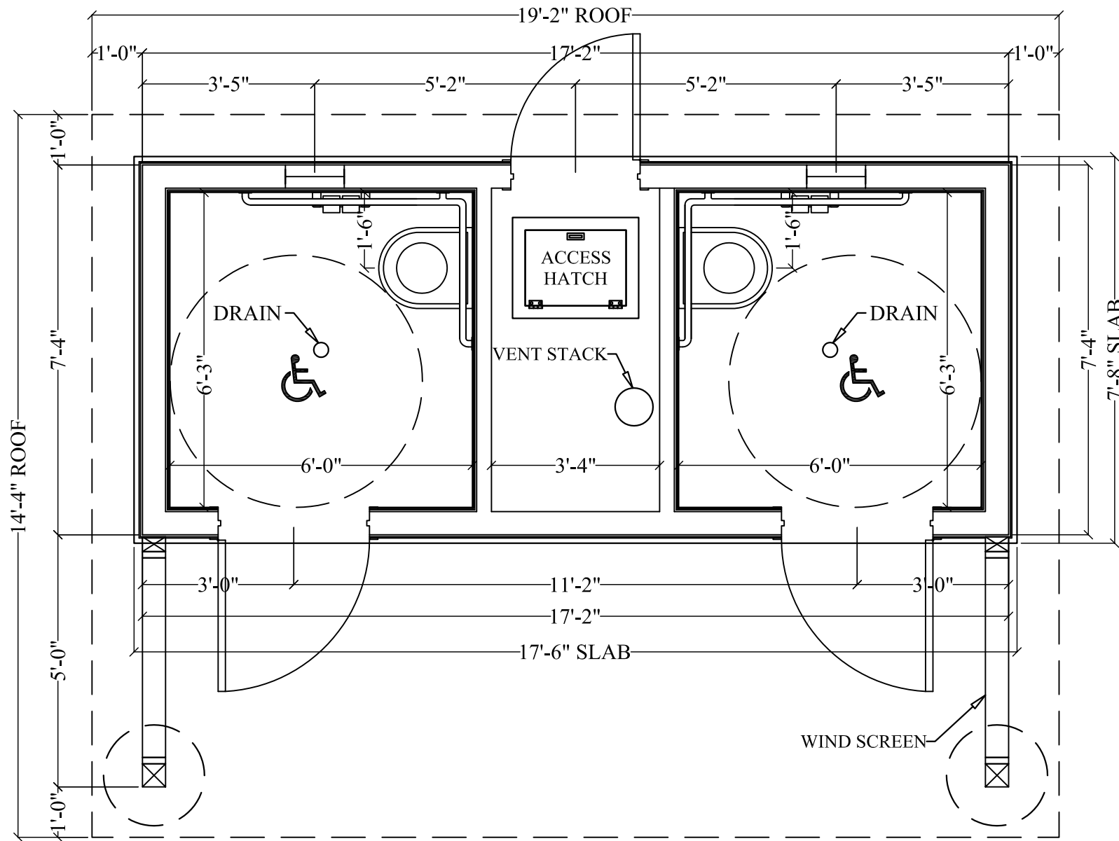
FLOOR PLAN
